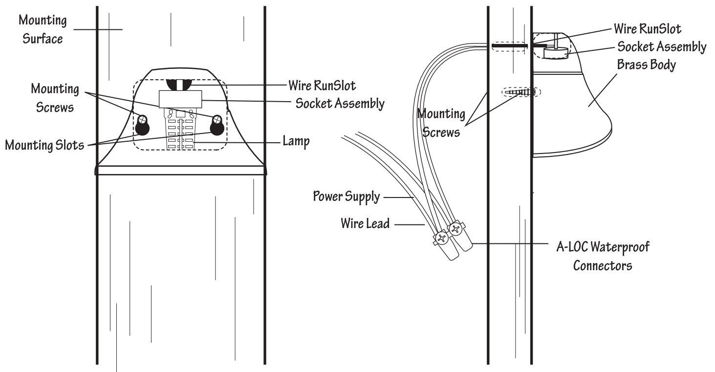
Front View
